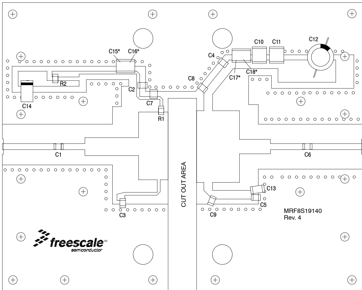
Figure 1. MRF8S19140HR3(HSR3) Test Circuit Component Layout
