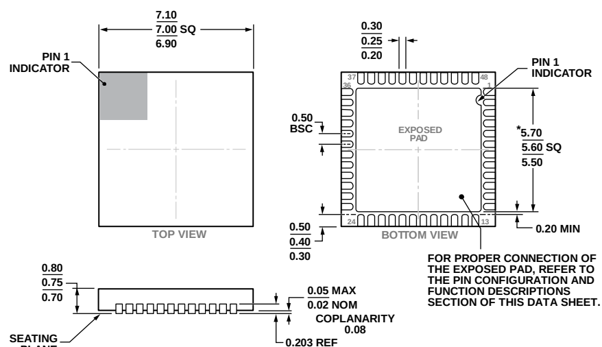
Figure 76. 48-Lead Lead Frame Chip Scale Package [LFCSP_WQ] 7 mm × 7 mm Body, Very Very Thin Quad (CP-48-13)
