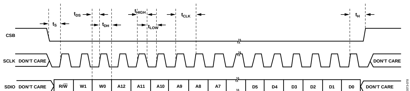
Figure 73. Serial Port Interface Timing Diagram
