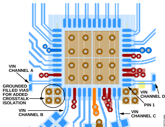
Figure 75. Layout Technique to Maximize Crosstalk Performance
