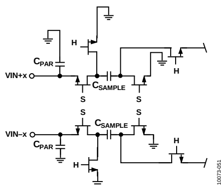
Figure 54. Switched-Capacitor Input Circuit
