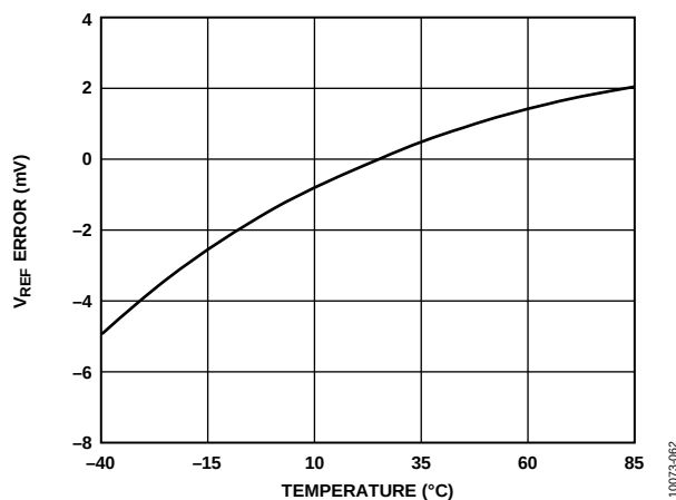
Figure 60. Typical V_{REF} Drift
