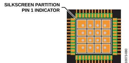
Figure 74. Typical PCB Layout
