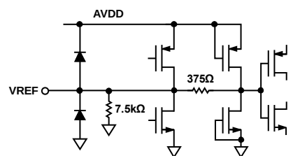
Figure 53. Equivalent VREF Circuit
