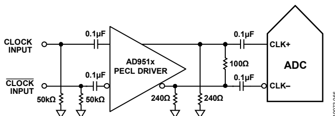
Figure 64. Differential PECL Sample Clock (Up to 1 GHz)
