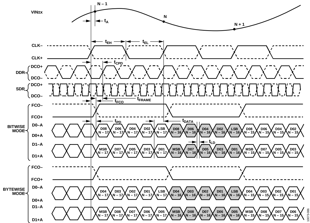
Figure 5. 10-Bit DDR/SDR, Two-Lane, 2x Frame Mode
