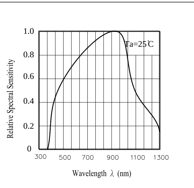
Spectral Sensitivity
