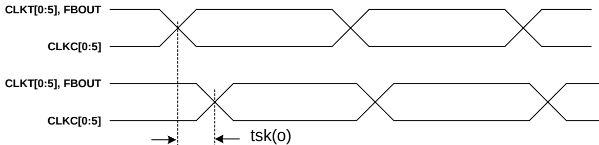
Figure 3. Output Skew
