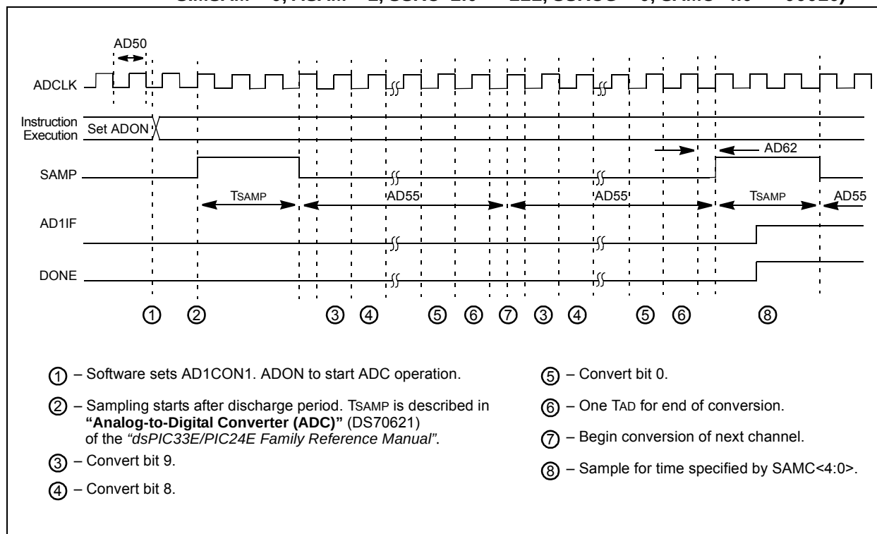
FIGURE 33-40: ADC CONVERSION (10-BIT MODE) TIMING CHARACTERISTICS (CHPS<1:0> = 01, SIMSAM = 0, ASAM = 1, SSRG<2:0> = 111, SSRG = 0, SAMC<4:0> = 00010)
