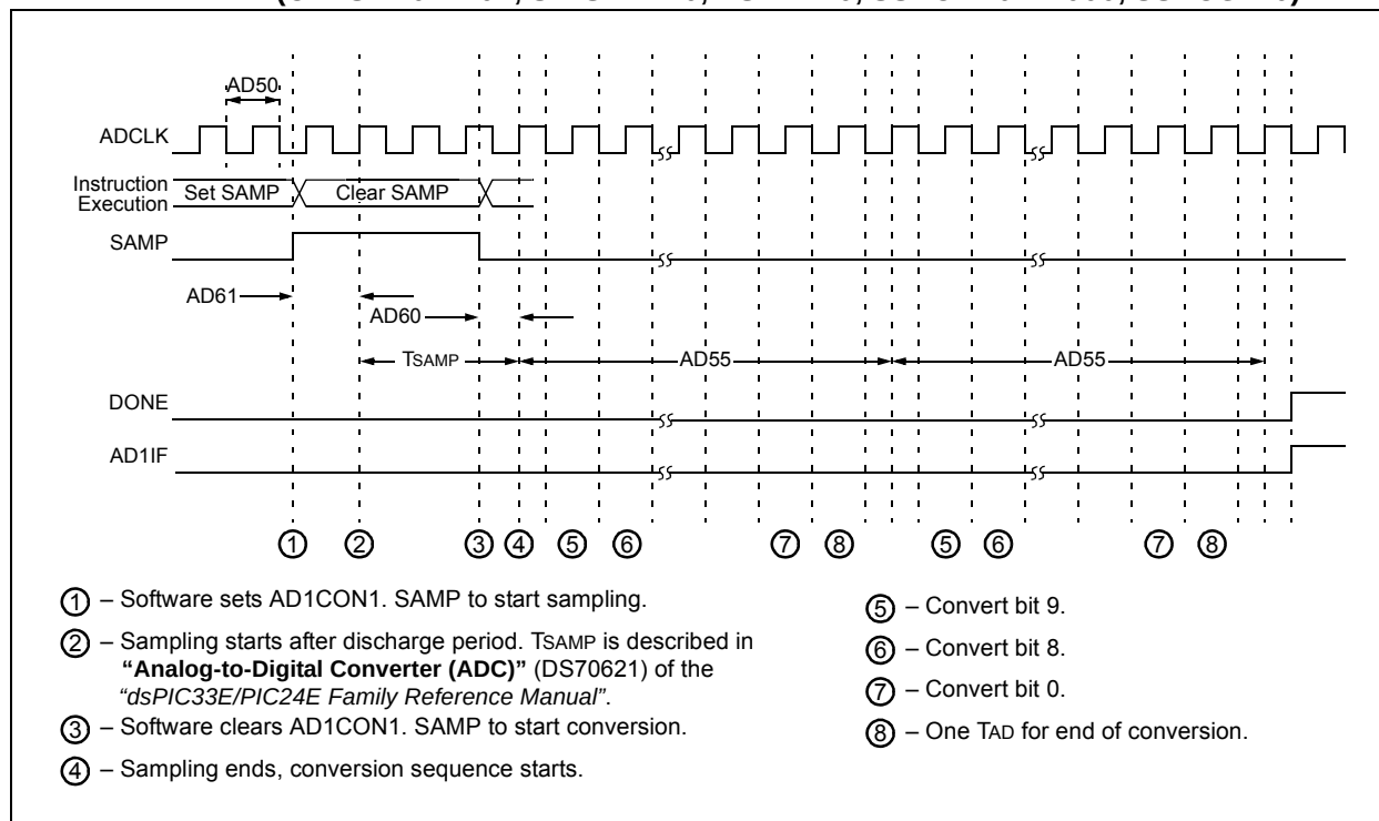
FIGURE 33-39: ADC CONVERSION (10-BIT MODE) TIMING CHARACTERISTICS (CHPS<1:0> = 01, SIMSAM = 0, ASAM = 0, SSRG<2:0> = 000, SSRG = 0)
