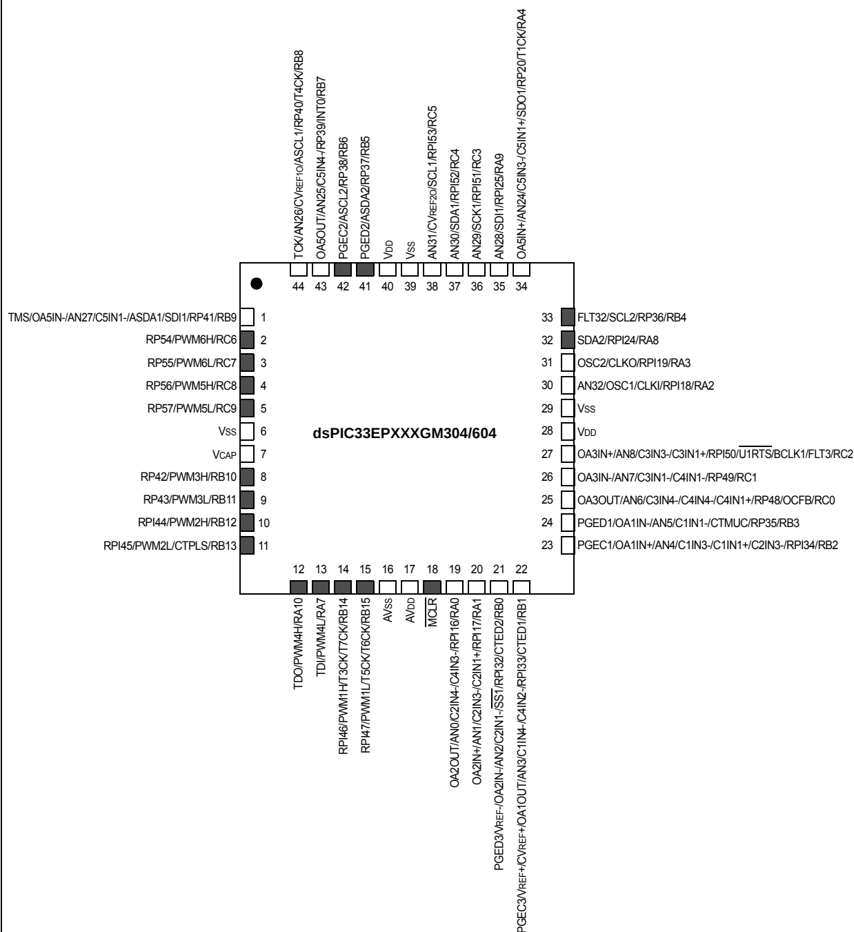
44-Pin QFN (1,2,3)
