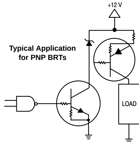
Figure 28. Inexpensive, Unregulated Current Source
