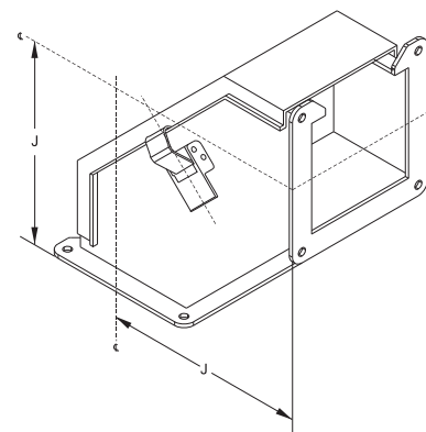
90° Elbow Outside Opening
