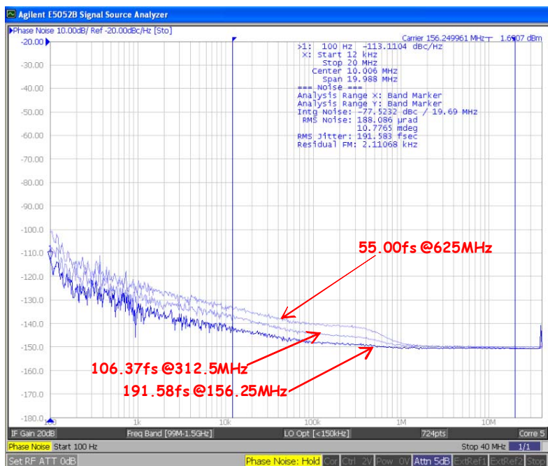
Total Jitter
