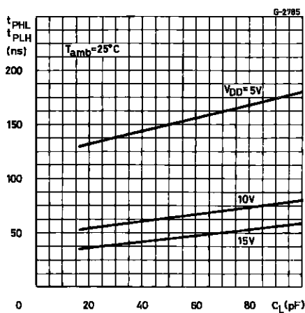
Typical Propagation Delay Time vs. Load Capacitance (CLOCK or SET to Q, CLOCK or RESET to \overline{Q} ).
