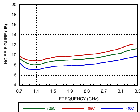
Figure 36. Noise Figure vs. Temperature @ VGATE=4.7V
