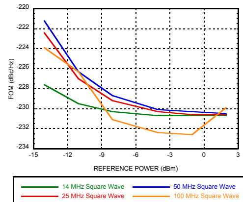
Figure 57. Reference Input Sensitivity, Square Wave, 50 \Omega [3]
