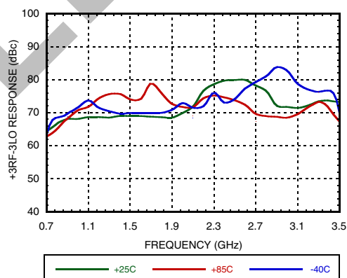
Figure 30. +3RF -3LO Response vs. Temperature @ VGATE=4.8V
