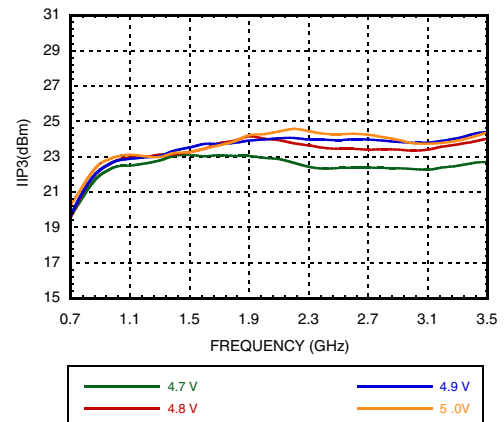
Figure 75. Conversion Gain & IIP3 vs. RF Frequency over VGATE Pin Voltage @25C, IF =150 MHz
