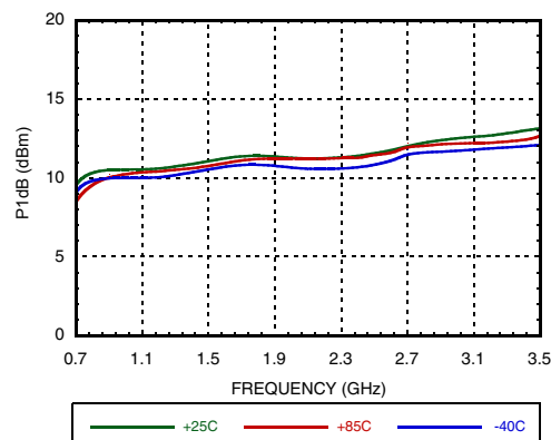
Figure 16. Input P1dB vs. Temperature @ VGATE=4.8V
