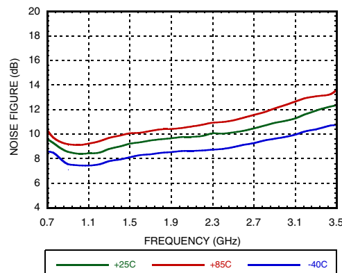
Figure 26. Noise Figure vs. Temperature @ VGATE=4.9V
