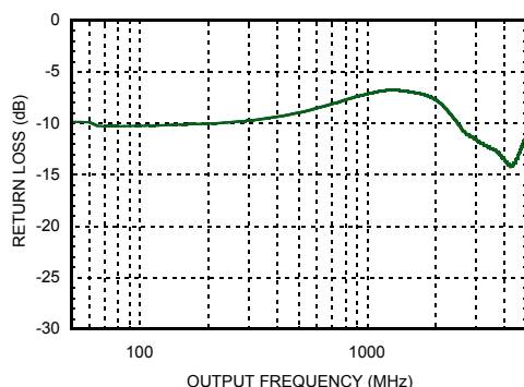
Figure 64. Auxiliary LO Differential Output Return Loss
