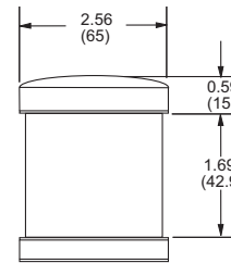
Alarm Unit Dimensions
