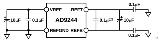
Figure 49. Reference Decoupling
