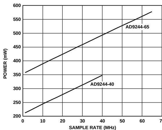
Figure 60. Power Consumption vs. Sample Rate
