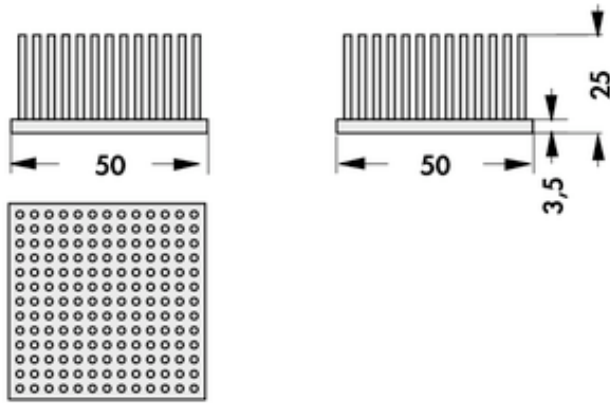
50 x 50 x 25 mm, pin heatsinks quadratic
