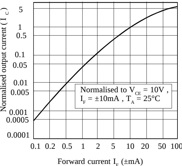
Normalised Output Current vs. Forward Current
