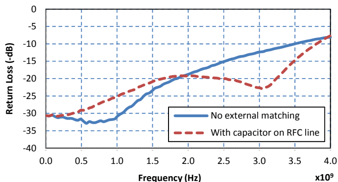
Figure 25. RFC Port Return Loss (RF2 Active) 1
