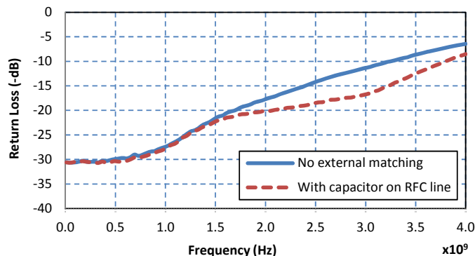
Figure 23. Active Port Return Loss (RF2 Active) 1
