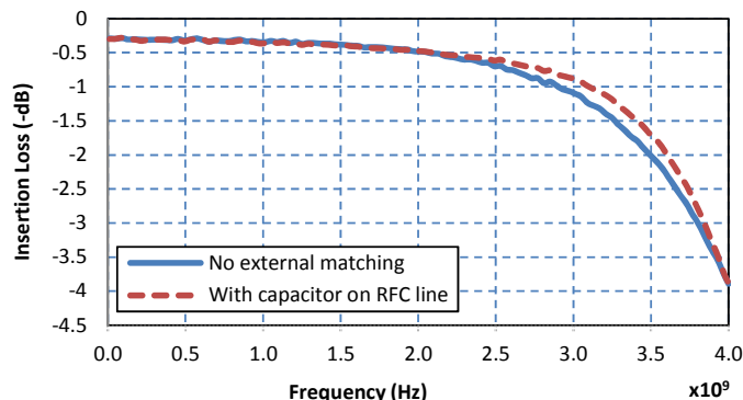
Figure 21. Insertion Loss RF2 1
