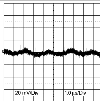
Figure 12. Output Ripple
