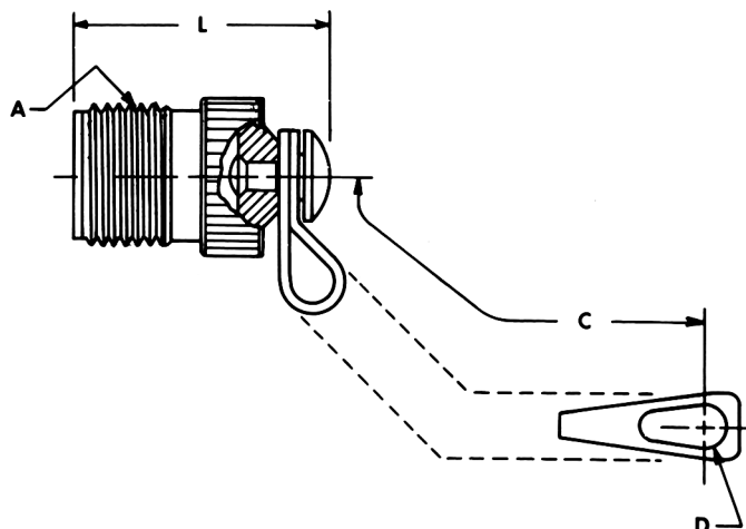
PLUG PROTECTION CAP MS25042-XXDA*
