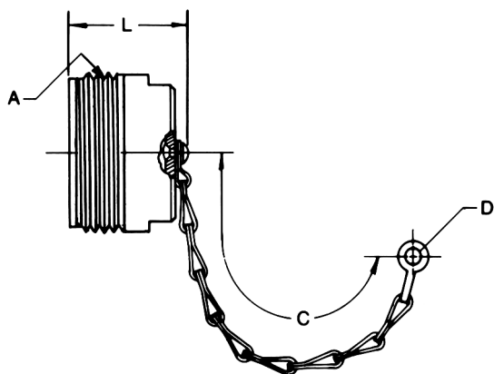
PLUG PROTECTION CAP MS25042-XXDA*
