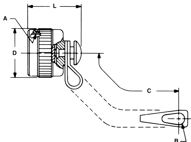
RECEPTACLE PROTECTION CAP MS25043-XXDA*
