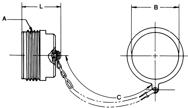
PLUG PROTECTION CAP 10-229125-XX*
