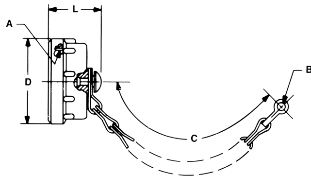
RECEPTACLE PROTECTION CAP 10-422905-XXX*
