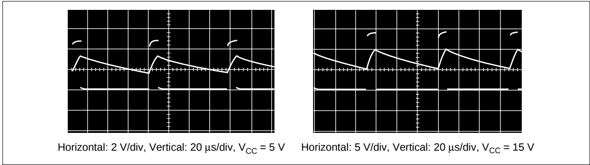
Figure 4 Operating Waveforms
