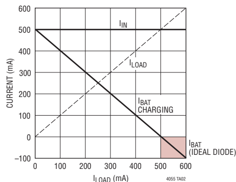
Input and Battery Current vs Load Current R_{PROG} = R_{CLPROG} = 97.6k
