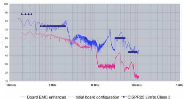
Figure 30. Conducted Emission Spectrum for 34981
