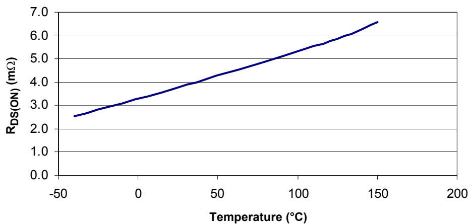
Figure 7. Typical R_{DS(ON)} vs. Temperature at V_{PWR} = 13 V
