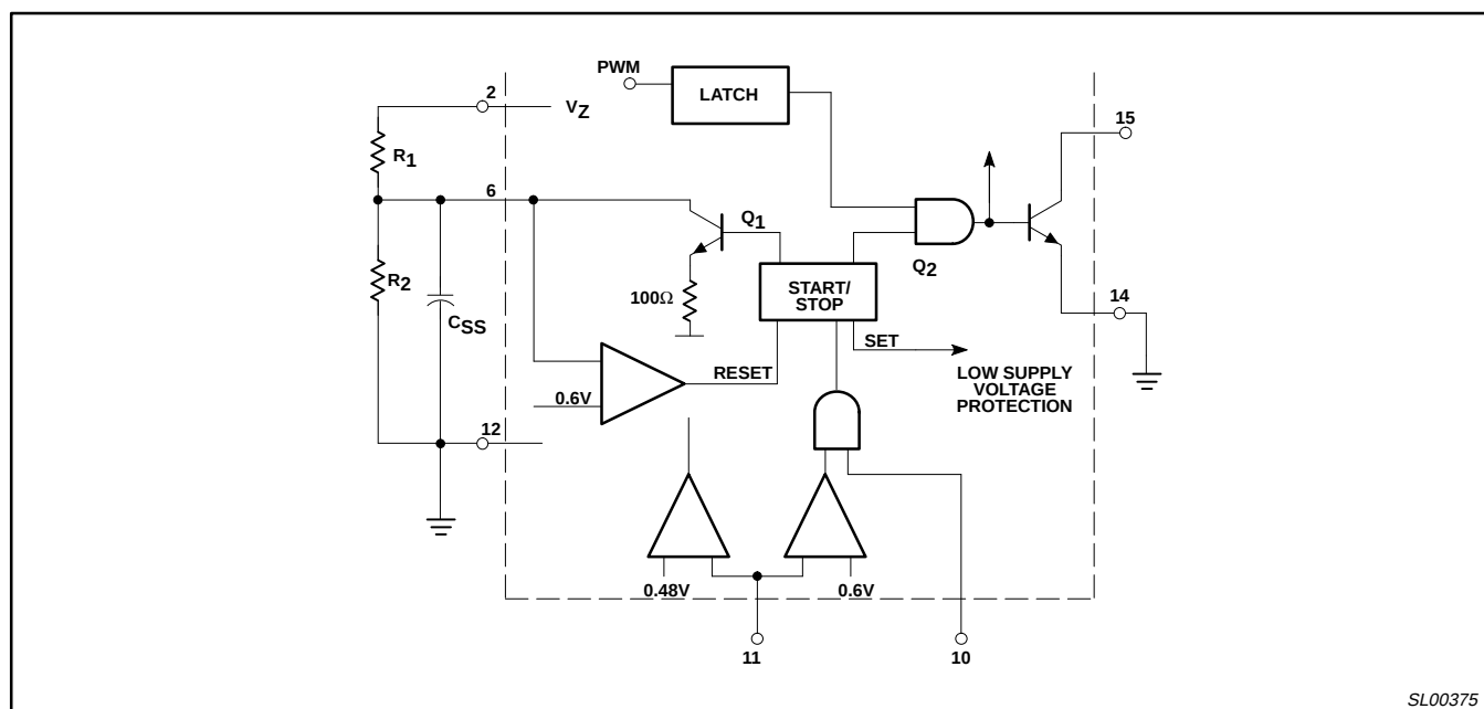
Figure 16. Start-Stop Circuit
