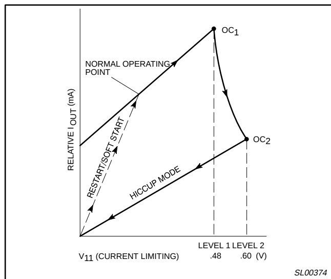
Figure 15. Output Characteristics
