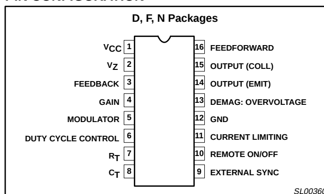
Figure 1. Pin Configuration
