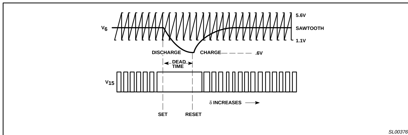
Figure 17. Start-Stop Circuit
