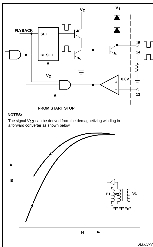
Figure 18. Output Stage
