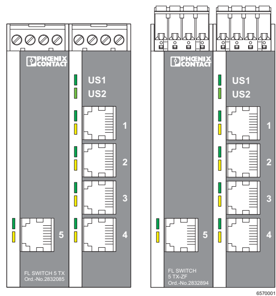
Figure 1 FL SWITCH 5TX (-ZF)
