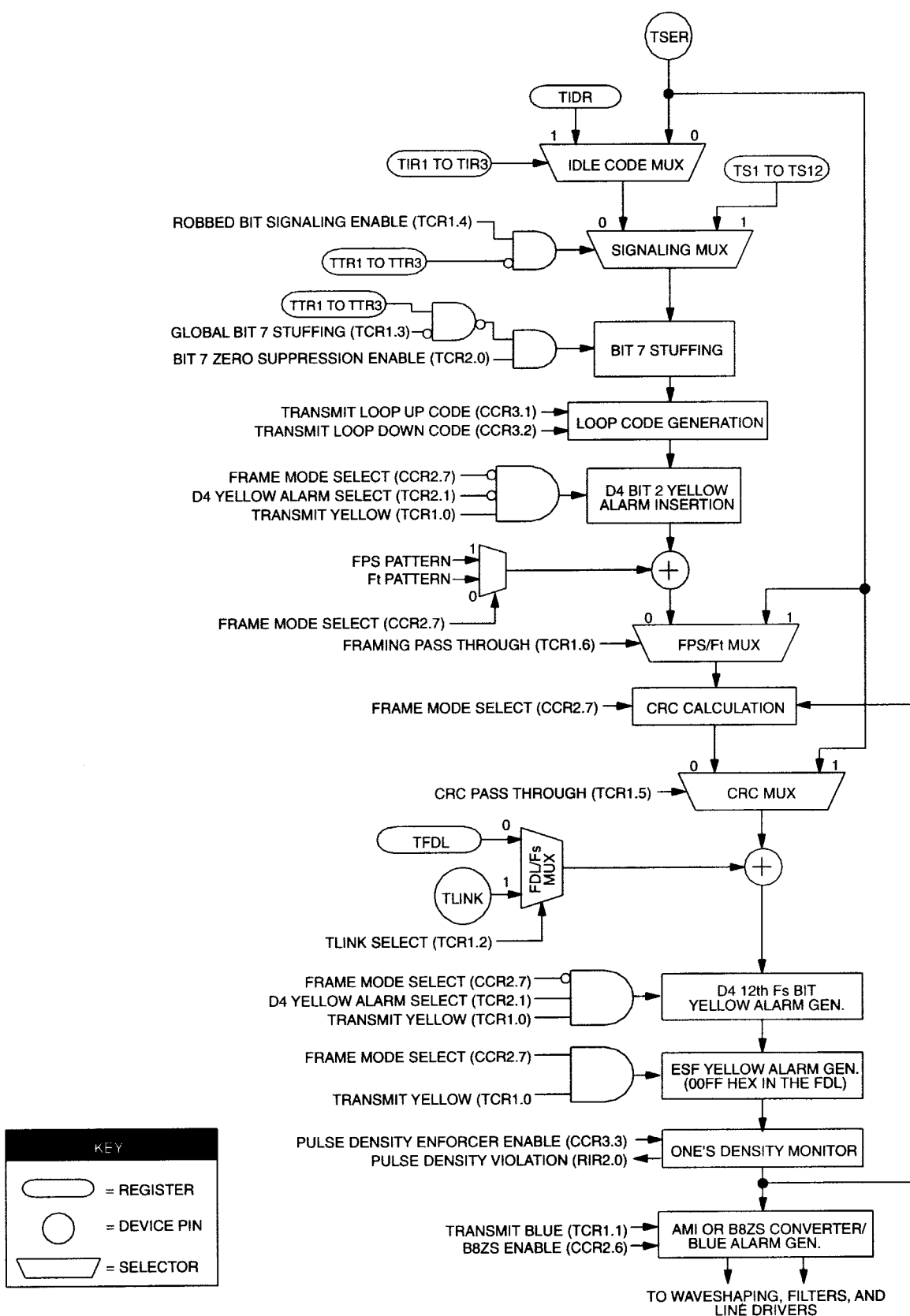
Figure 14-9. Transmit Data Flow
