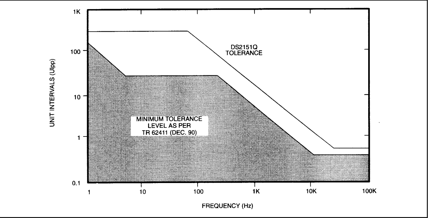
Figure 13-2. Jitter Tolerance
