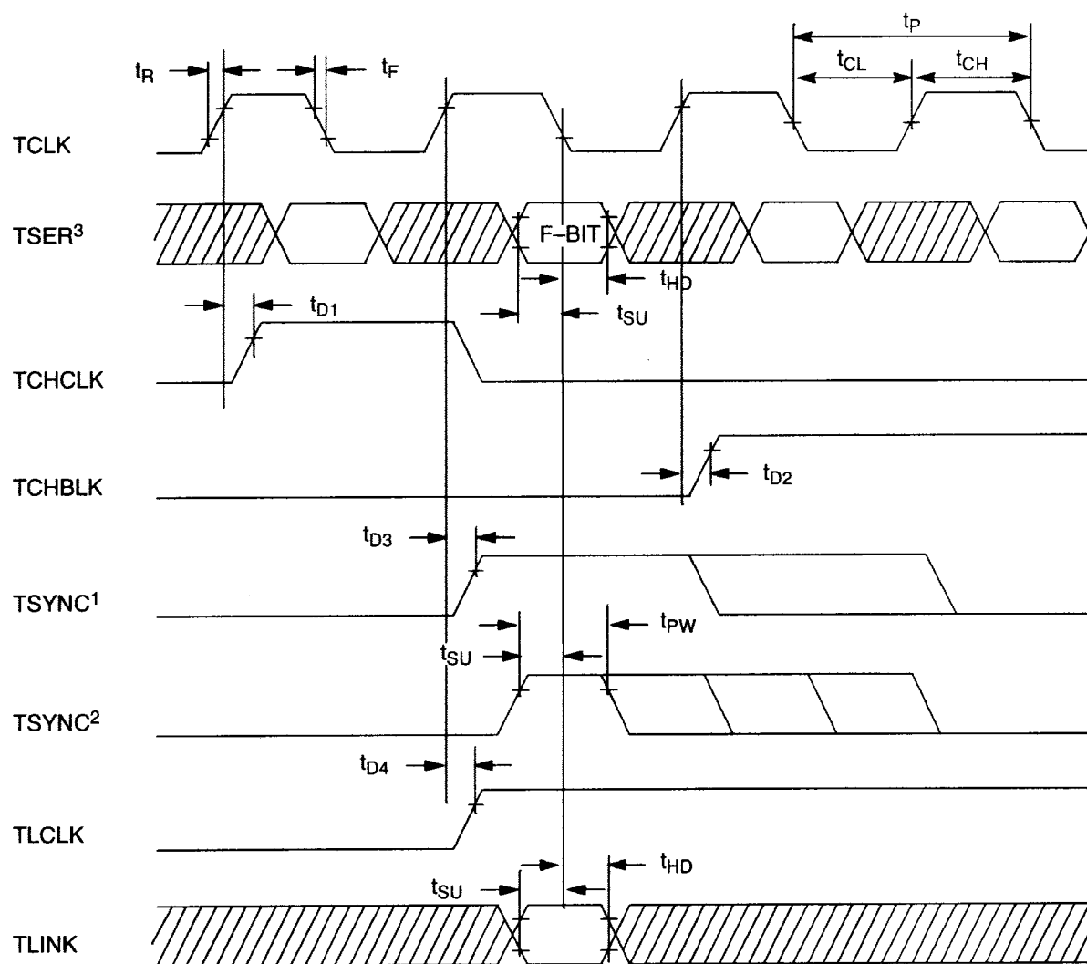
Figure 16-5. Transmit Side AC Timing
