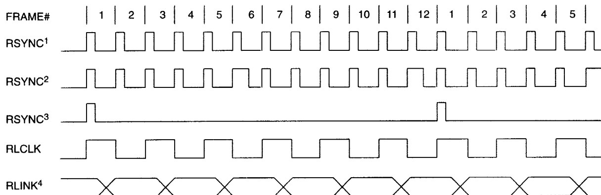
Figure 14-1. Receive Side D4 Timing
