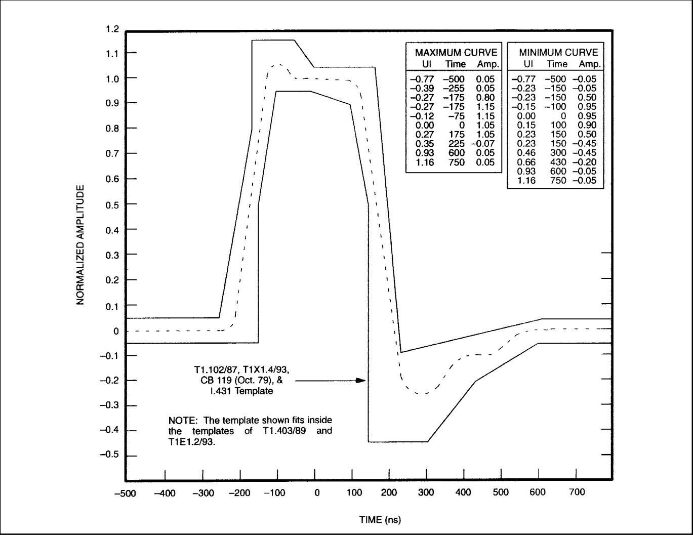
Figure 13-3. Transmit Waveform Template
