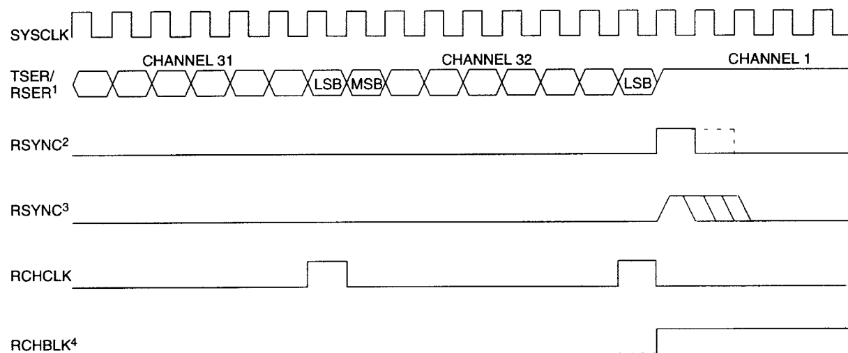
Figure 14-5. 2.048MHz Boundary Timing with Elastic Store(s) Enabled
