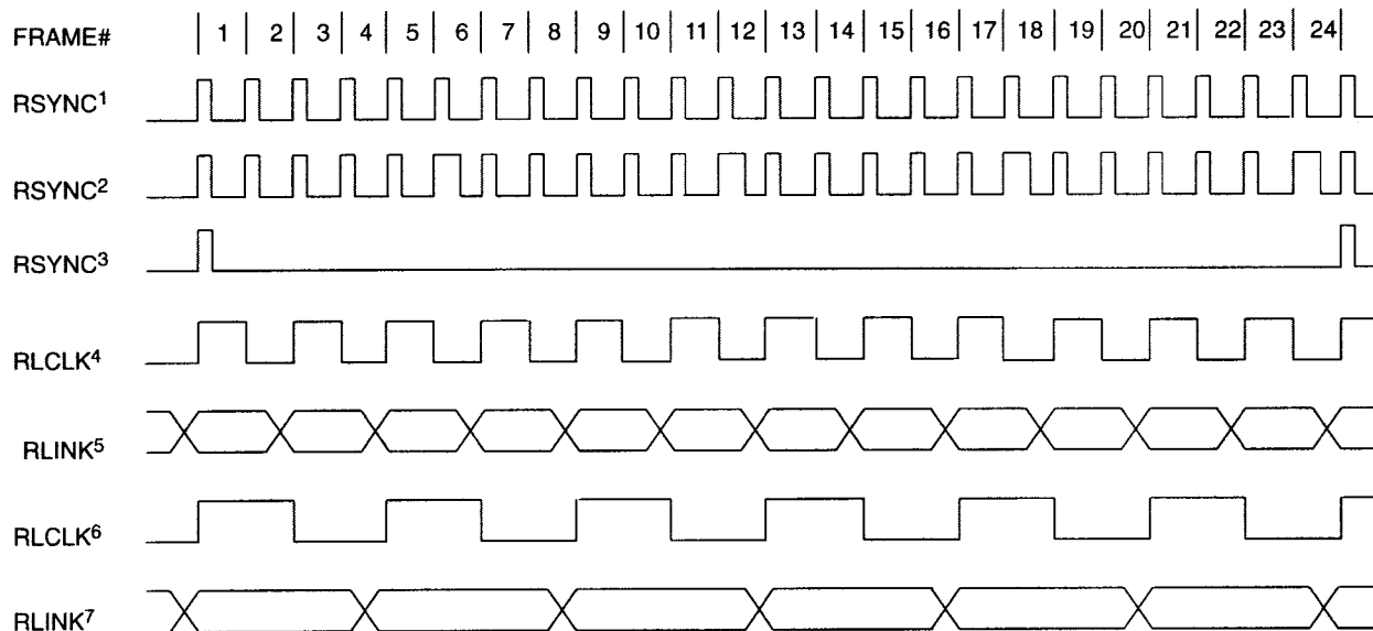
Figure 14-2. Receive Side ESF Timing
