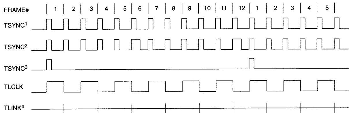
Figure 14-6. Transmit Side D4 Timing
