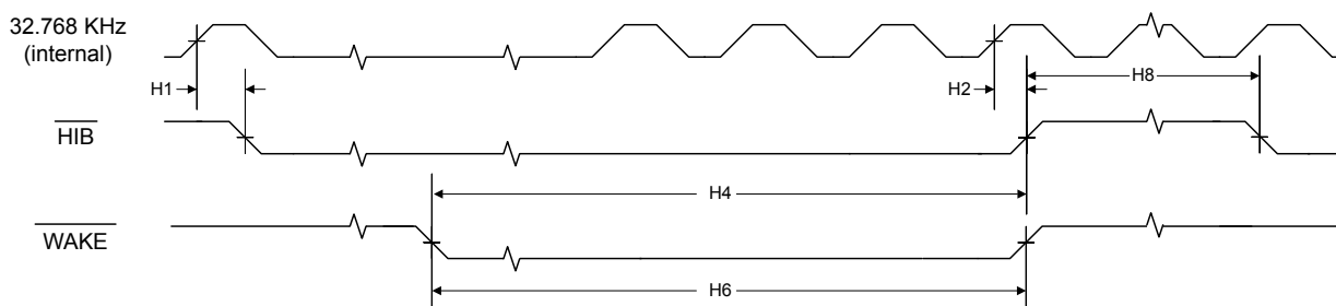
Figure 26-12. Hibernation Module Timing with Internal Oscillator Stopped in Hibernation
