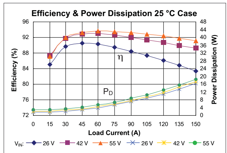
Figure 4 — Efficiency and power dissipation at 25\text{ }^{\circ}\text{C}
