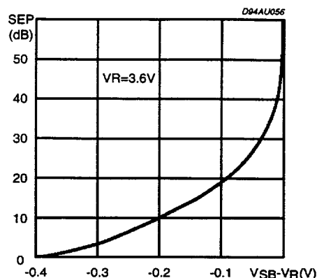
Figure 2: Stereo Blend
