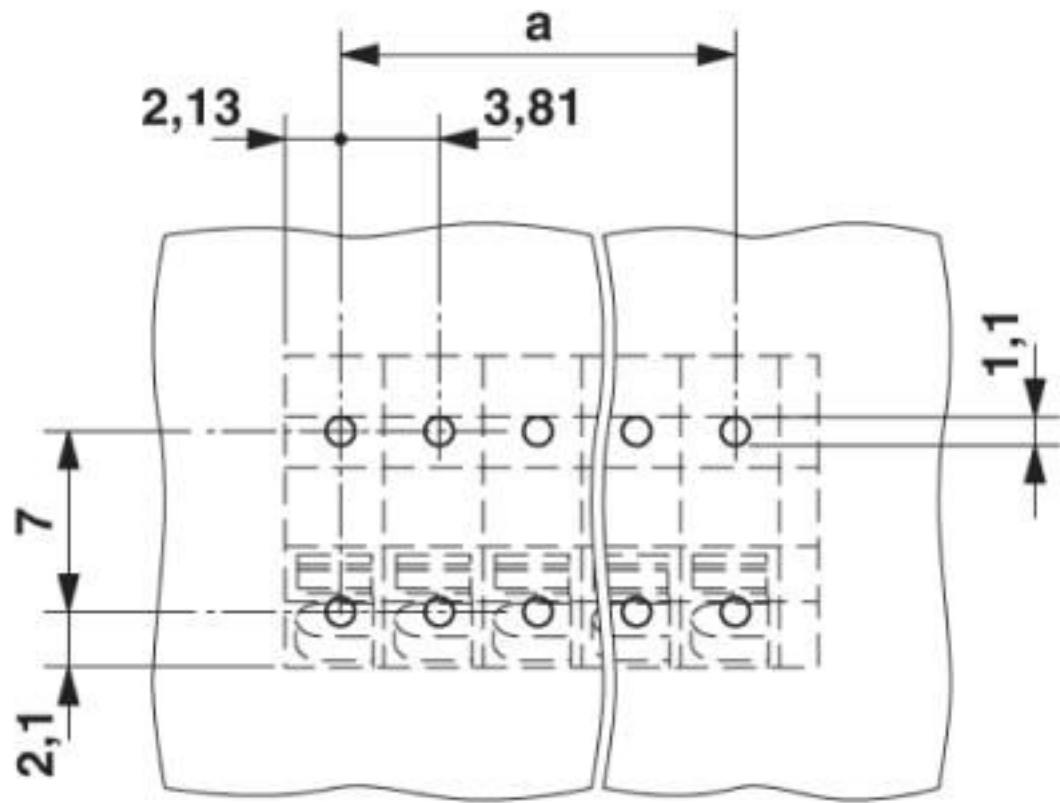
Drilling diagram
