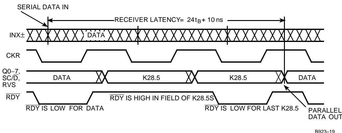
Figure 3. CY7B933 Receiver Data Pipeline in Encoded Mode
