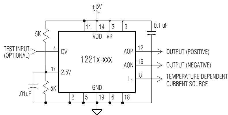
RECOMMENDED CONNECTIONS
