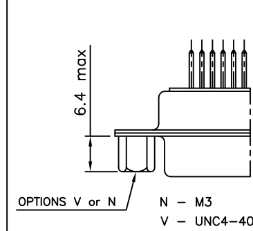
HEXAGONAL FEMALE SCREW
