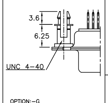
HARPOON RIVETTED TO SHELL
