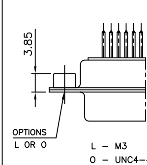
CLINCH NUT
