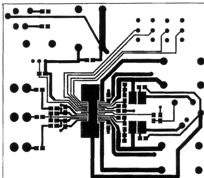
Figure 48. Top Layer TSSOP
