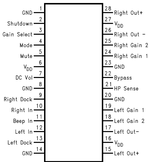
Figure 2. HTSSOP Package (Top View) See Package Number PWP0028A for HTSSOP
