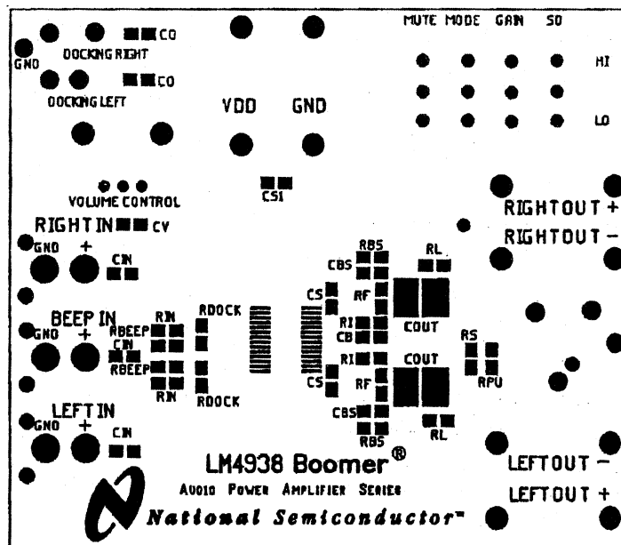
Figure 47. Top Layer Silkscreen
