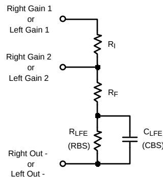
Figure 46. Low Frequency Enhancement
