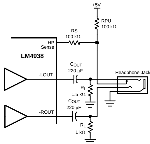
Figure 45. Headphone Sensing Circuit
