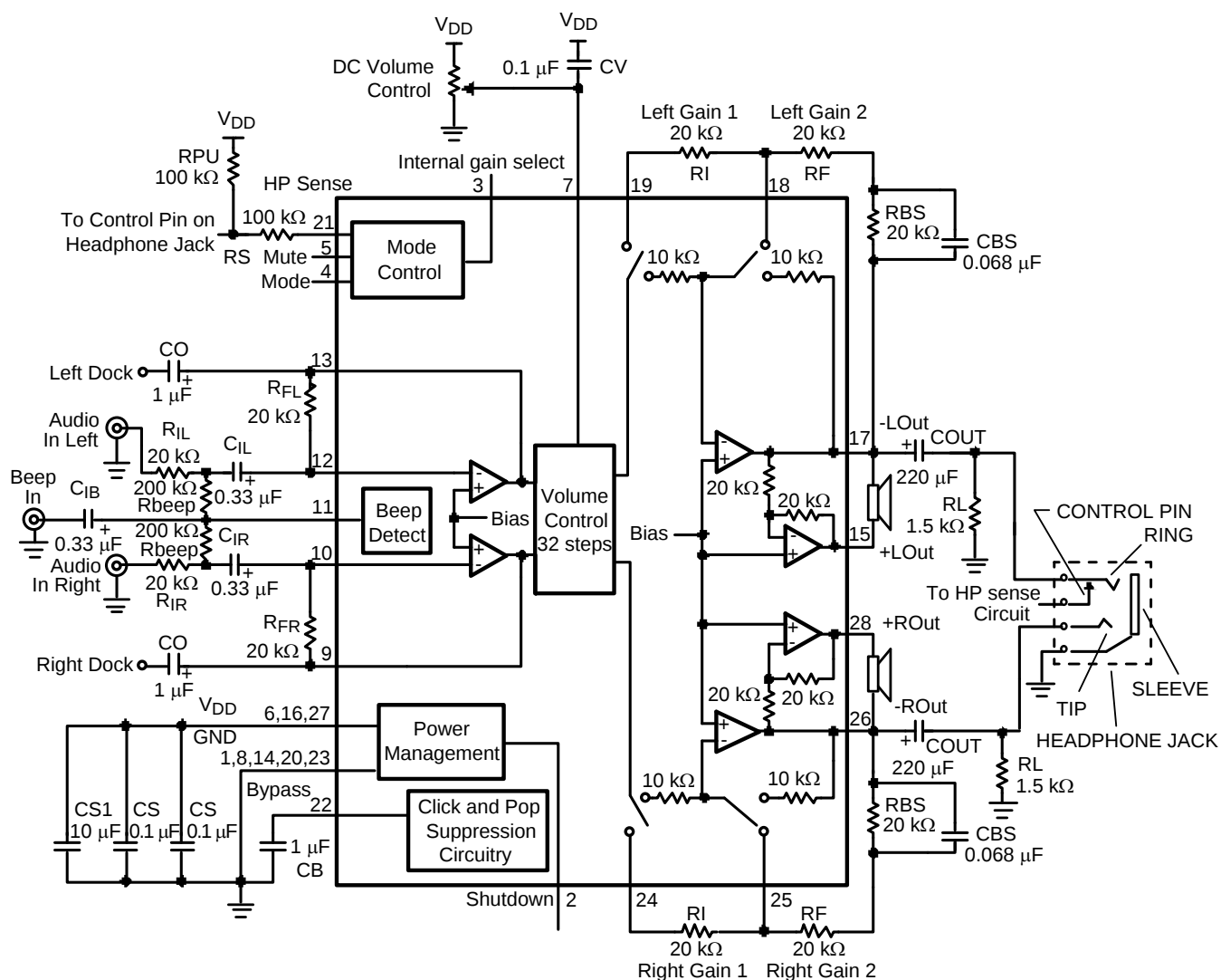
Figure 3. Typical Application Circuit
