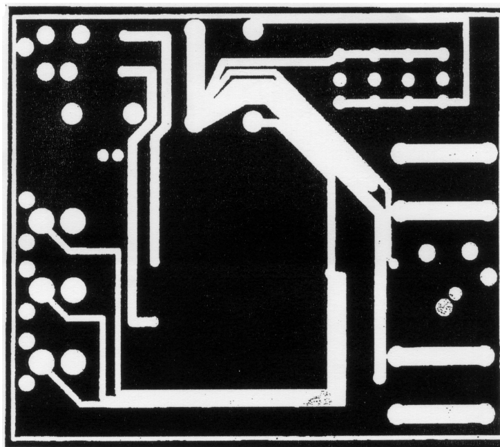
Figure 50. Inner Layer (3)
