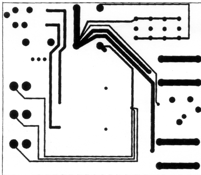
Figure 51. Bottom Layer TSSOP
