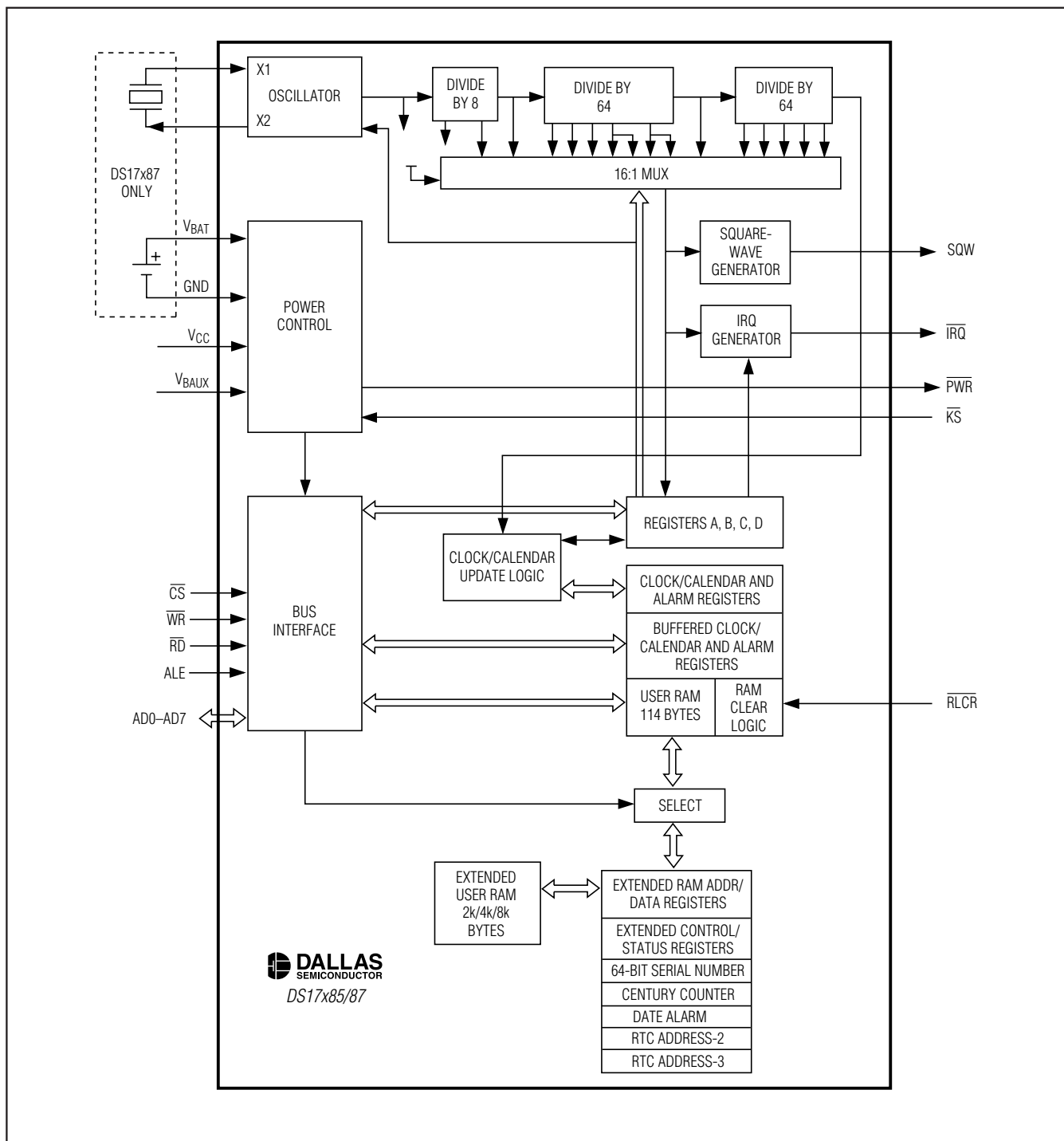
Figure 1. Functional Diagram
