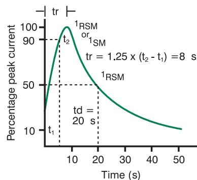
8/20 \mu S IMPULSE DISCHARGE CURRENT WAVESHAP
