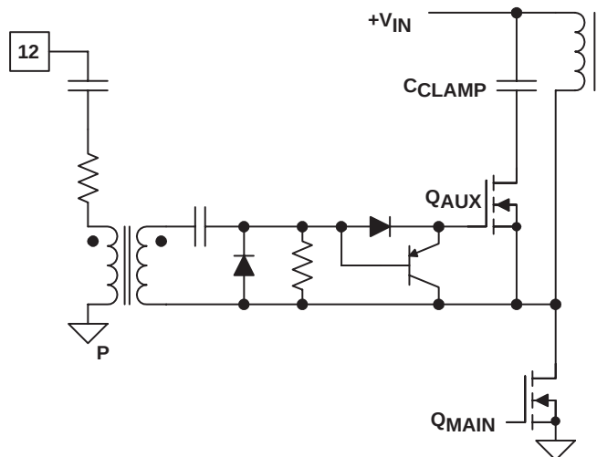
Interfacing with a high side N-channel clamp switch is achievable by using high side gate drive integrated circuits or through a gate drive transformer. When a transformer is used, special attention must be paid to the fact that the clamp switch is operated by the complementary waveform of the main power switch. Since the operating duty cycle of the converter can vary between 0 and D_{MAX} , the gate drive transformer must be able to drive the auxiliary switch with any duty cycle from 1-D_{MAX} to near 1.
