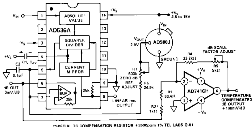
Figure 10. dB Connection
