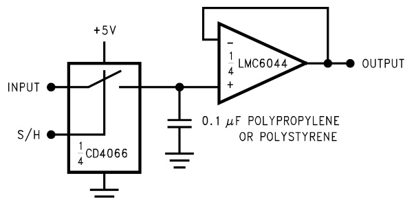
Figure 37. Low-Leakage Sample-and-Hold
