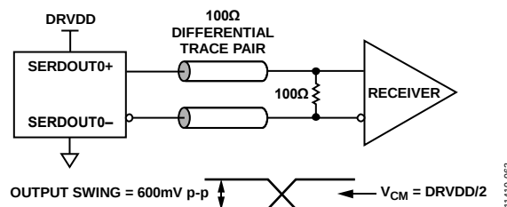
Figure 63. DC-Coupled Digital Output Termination Example
