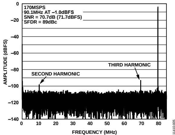
Figure 5. AD9683-170 Single-Tone FFT with f_{IN} = 90.1 MHz
