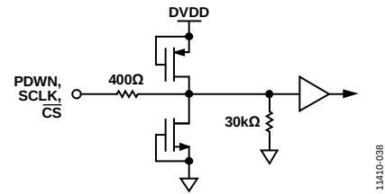
Figure 38. Equivalent PDWN, SCLK, or \overline{CS} Input Circuit
