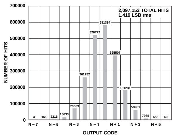
Figure 32. AD9683-250 Grounded Input Histogram
