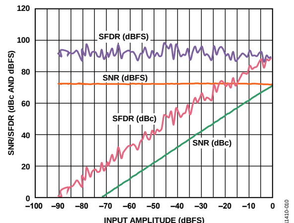
Figure 10. AD9683-170 Single-Tone SNR/SFDR vs. Input Amplitude ( A_{IN} ) with f_{IN} = 185.1 MHz
