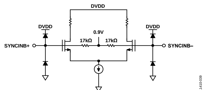
Figure 39. Equivalent SYNCINB± Input Circuit
