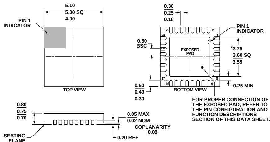
Figure 68. 32-Lead Lead Frame Chip Scale Package [LFCSP_WQ] 5 mm × 5 mm Body, Very Very Thin Quad (CP-32-12) Dimensions shown in millimeters
