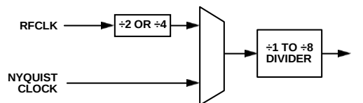
Figure 55. Clock Divider Circuit
