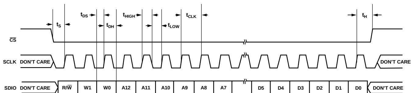
Figure 67. Serial Port Interface Timing Diagram
