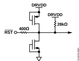
Figure 41. Equivalent \overline{RST} Input Circuit
