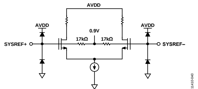
Figure 40. Equivalent SYSREF± Input Circuit
