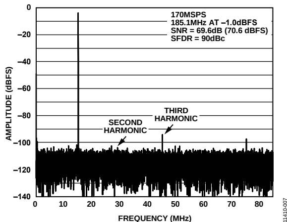
Figure 7. AD9683-170 Single-Tone FFT with f_{IN} = 185.1 MHz
