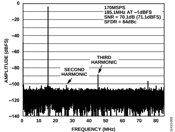
Figure 8. AD9683-170 Single-Tone FFT with f_{IN} = 185.1 MHz, RFCLK = 680 MHz with Divide by 4 (Address 0x09 = 0x21)
