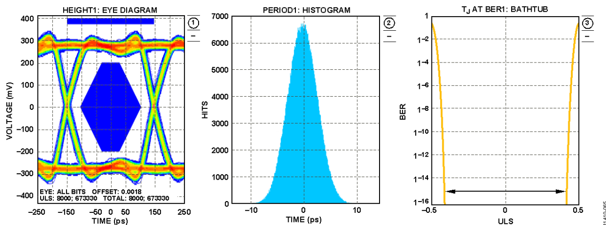
Figure 65. AD9683 Digital Outputs Data Eye, Histogram and Bathtub, External 100 Ω Terminations at 3.4 Gbps
