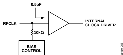
Figure 53. Equivalent RF Clock Input Circuit
