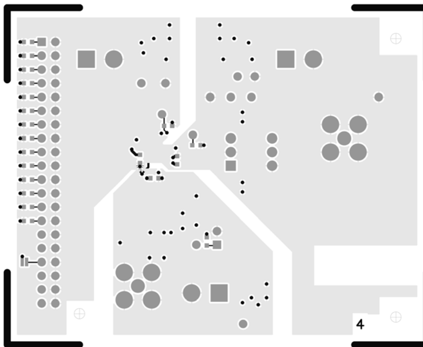
Figure 23. Evaluation Board Layout: Secondary Side
