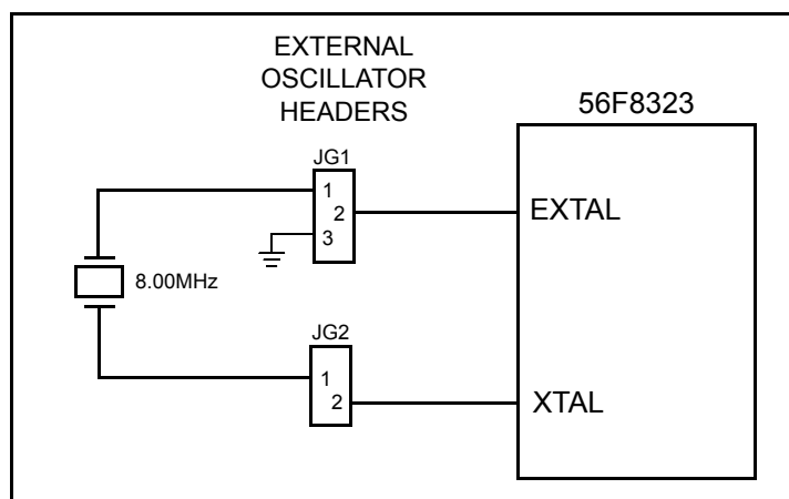
Figure 2-2. Schematic Diagram of the Clock Interface
