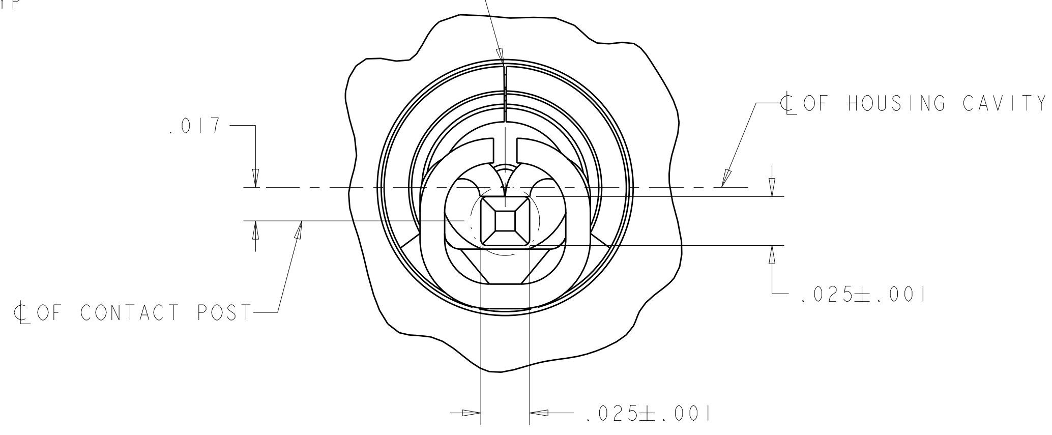
DETAIL V SCALE 20:1
