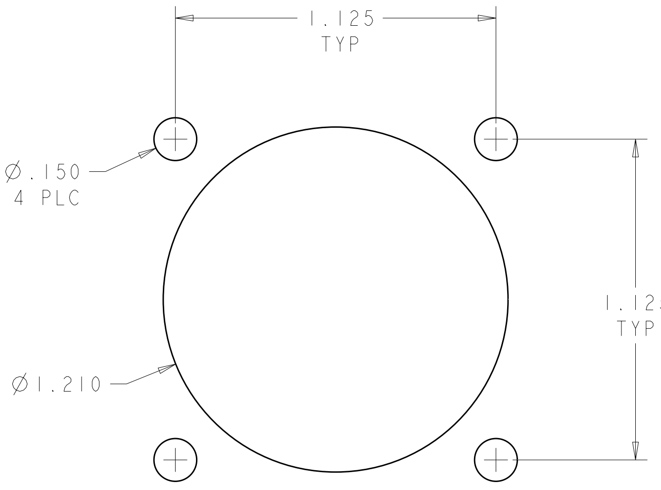
RECOMMENDED PANEL LAYOUT .125 MAX PANEL THICKNESS SCALE 3:1
