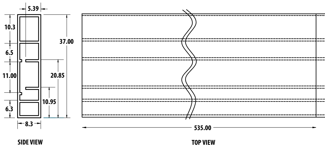
Figure 13. Tube dimensions
