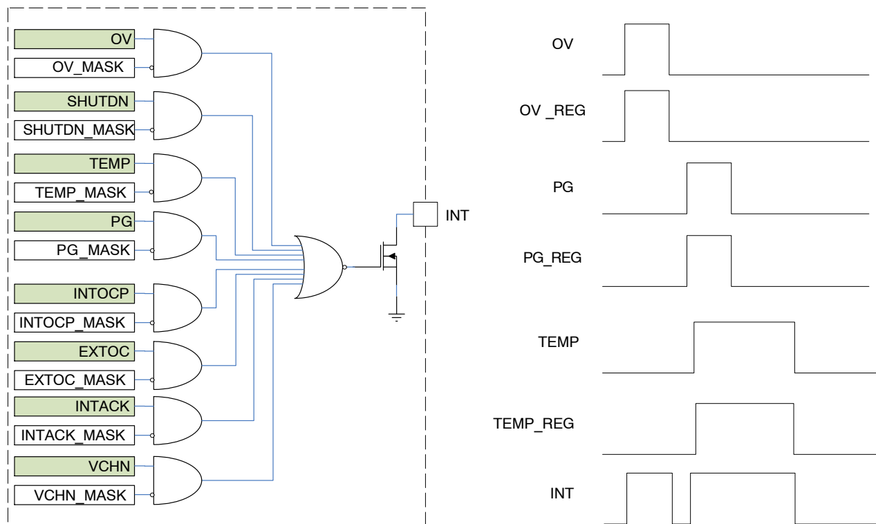
Figure 15. Interrupt Logic
