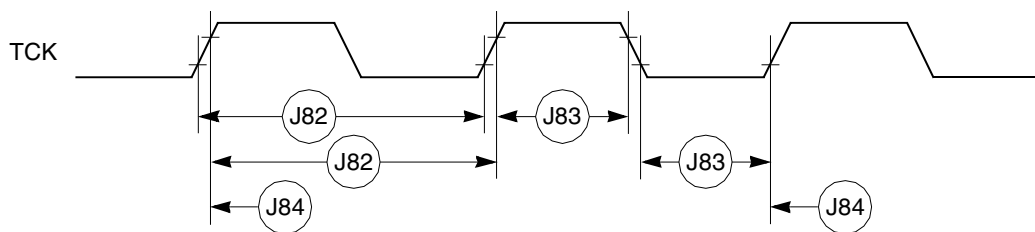
Figure 38. JTAG Test Clock Input Timing
