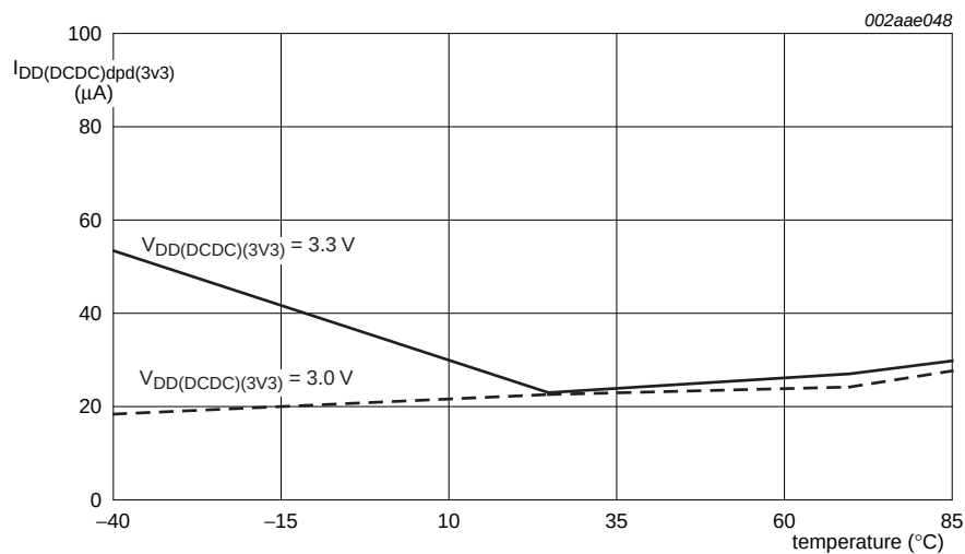
Fig 10. Total DC-to-DC converter maximum supply current I_{DD(DCDC)dcpd(3v3)} versus temperature in Deep power-down mode
