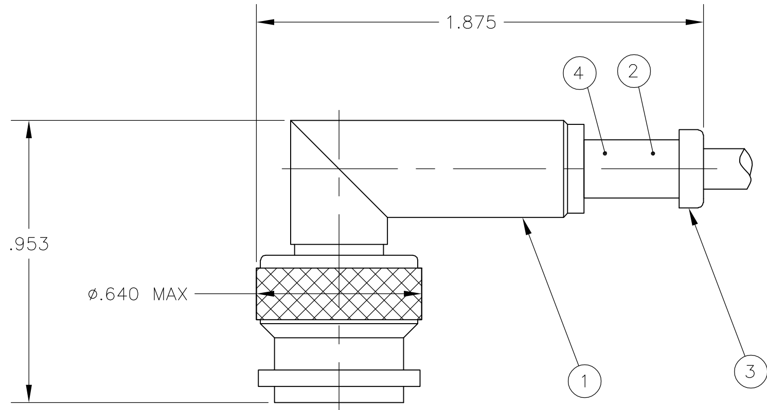
ASSEMBLED VIEW
