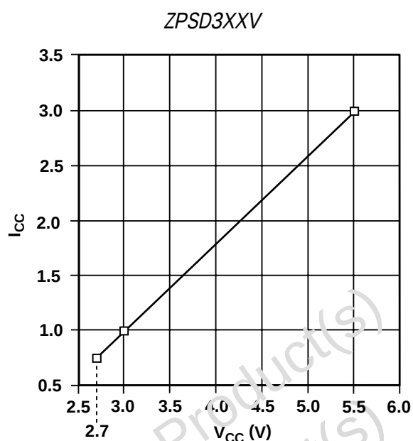
Figure 17. Normalized I_{CC} (DC vs. V_{CC} ) ( V_{CC} = 3.0\text{ V} )
