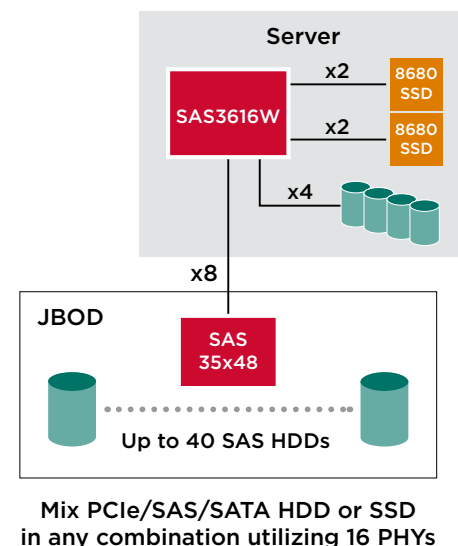
Figure 2: Direct Attached PCIe SSDs and SAS/SATA HDD combined with an expander to SAS/SATA HDDs
