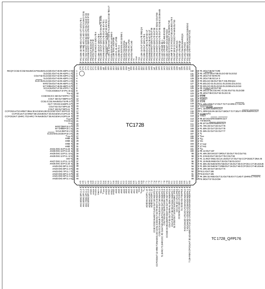
Figure 3-2 SAK-TC1728N-192F133HL / SAK-TC1728N-192F133HR Pinning
