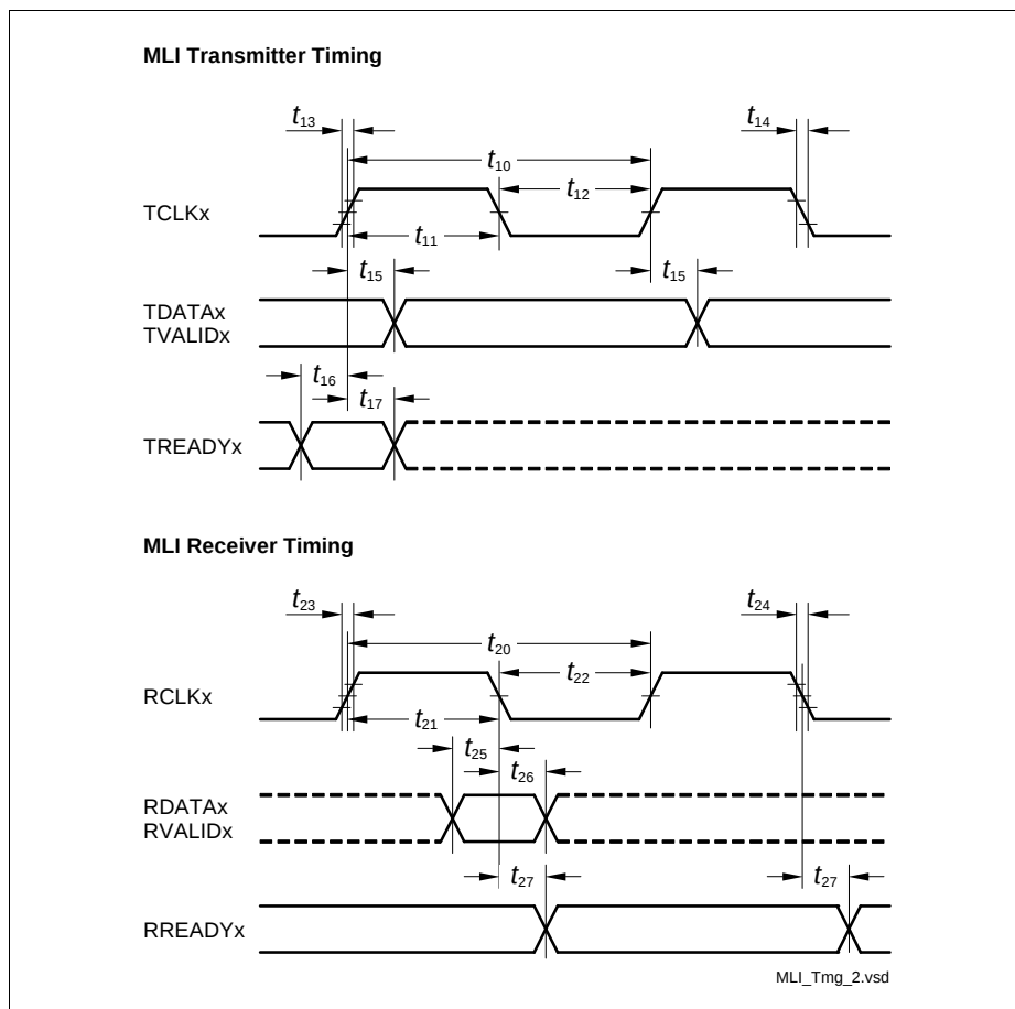
Figure 17 MLI Interface Timing
