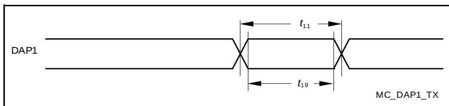
Figure 16 DAP Timing Device to Host
