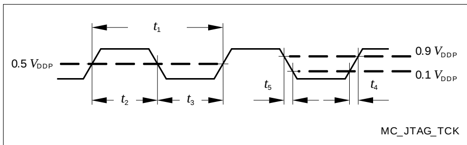
Figure 12 Test Clock Timing (TCK)
