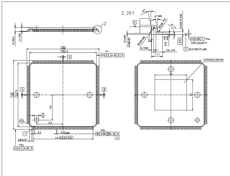
Figure 21 Package Outlines PG-LQFP-176-10
