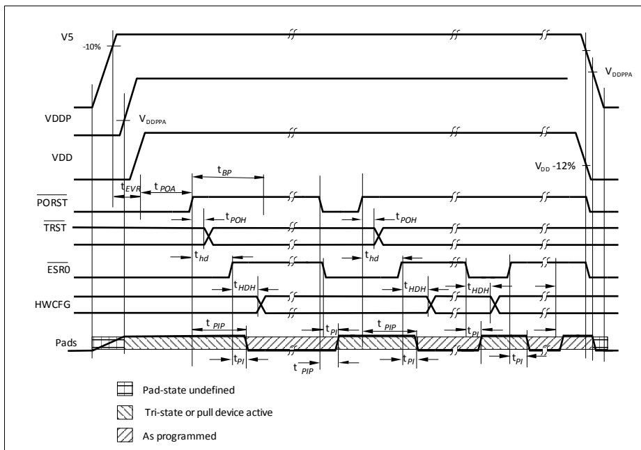
Figure 11 Power, Pad and Reset Timing
