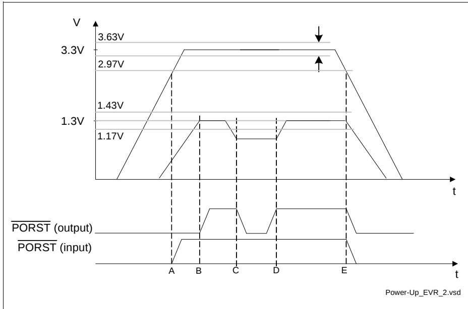
Figure 9 3.3 V / 1.3 V Power-Up/Down Sequence
