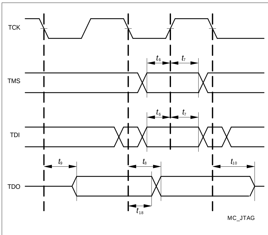
Figure 13 JTAG Timing
