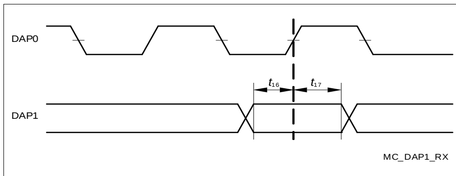
Figure 15 DAP Timing Host to Device
