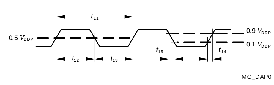
Figure 14 Test Clock Timing (DAP0)
