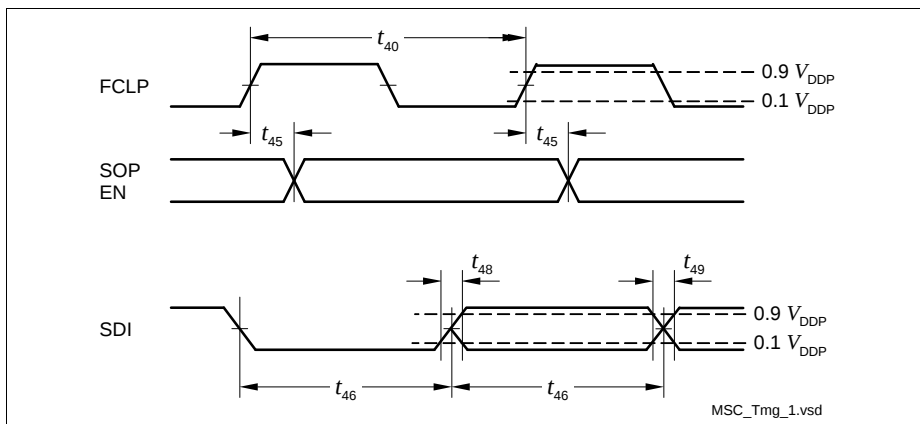
Figure 18 MSC Interface Timing
