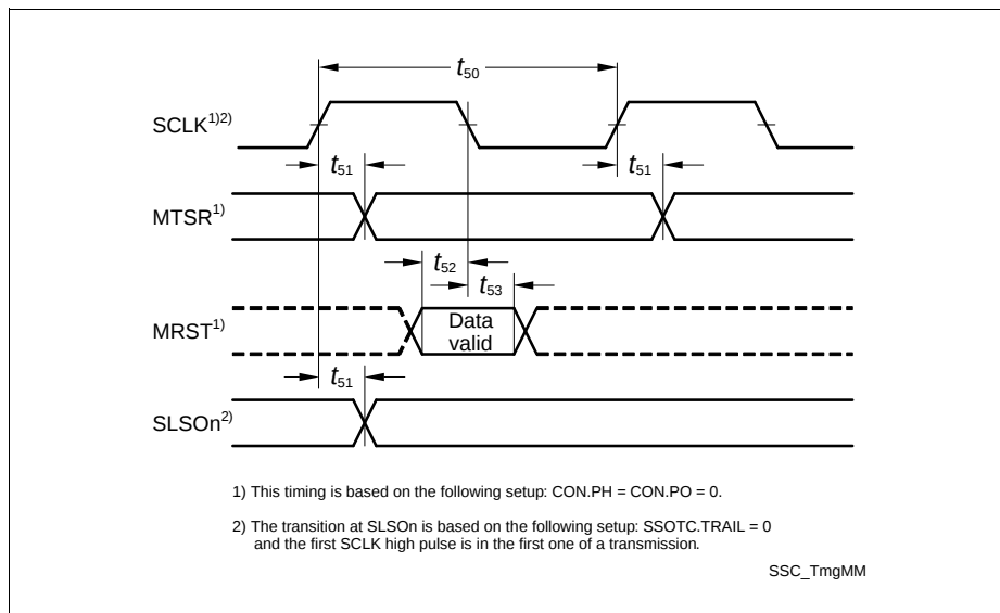
Figure 19 Master Mode Timing
