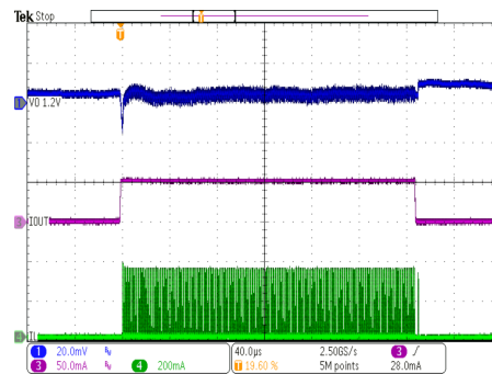
TPS62801 V_{OUT} = 1.2\text{ V} VSEL/MODE = GND rise / fall time < 1 I_{OUT} = 0\text{ mA to } 50\text{ mA} , PFM Mode \mu\text{s}
