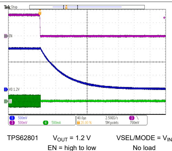
Figure 8-41. Output Discharge
