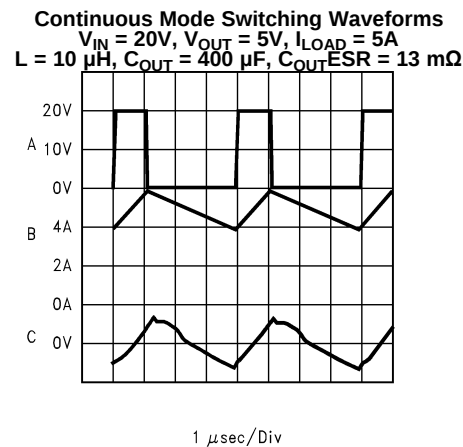
A: V_{\text{SW}} Pin Voltage, 10 V/div. B: Inductor Current, 2 A/div C: Output Ripple Voltage, 20 mV/div AC-Coupled Figure 15. Horizontal Time Base: 1 \mu\text{s/div}
